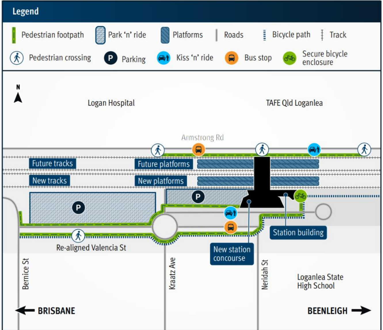
Site layout map – Loganlea Station Relocation project
